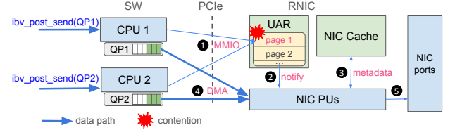
Figure 6: Data verbs cause severe UAR contention.
